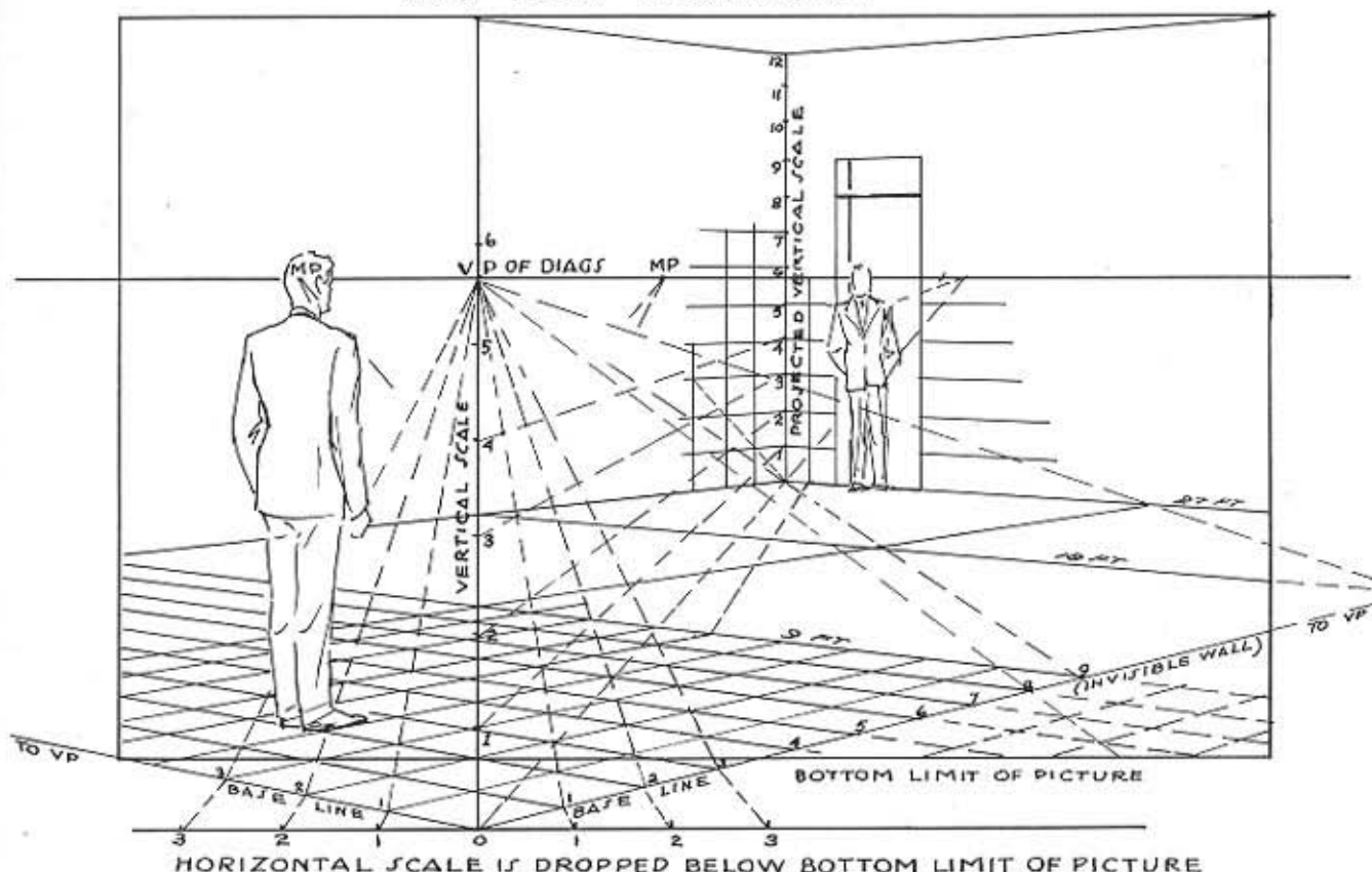
TWO - POINT PERSPECTIVE
